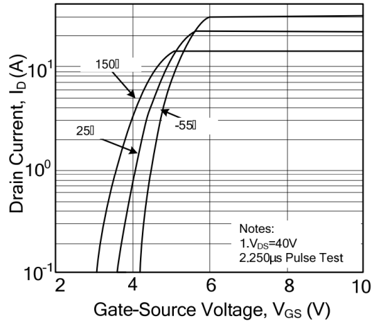
4. Transfer Characteristics
